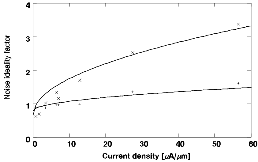
Figure 3.10a: Noise ideality factor ( \alpha ) as a function of current density ( I/W ) for buried channel type ((+): \delta L=0.06 \mu\text{m} ) and surface channel type ((x): \delta L=0.39 \mu\text{m} ). The channel length L is fixed.
