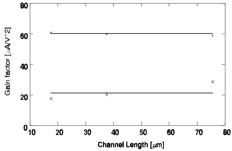
Figure 3.9b: Gain factor \mu_n C_{\square} of a buried channel (x) and surface channel (+) transistor as a function of channel length L_1 . The channel width W_1 and bias current I are fixed.
