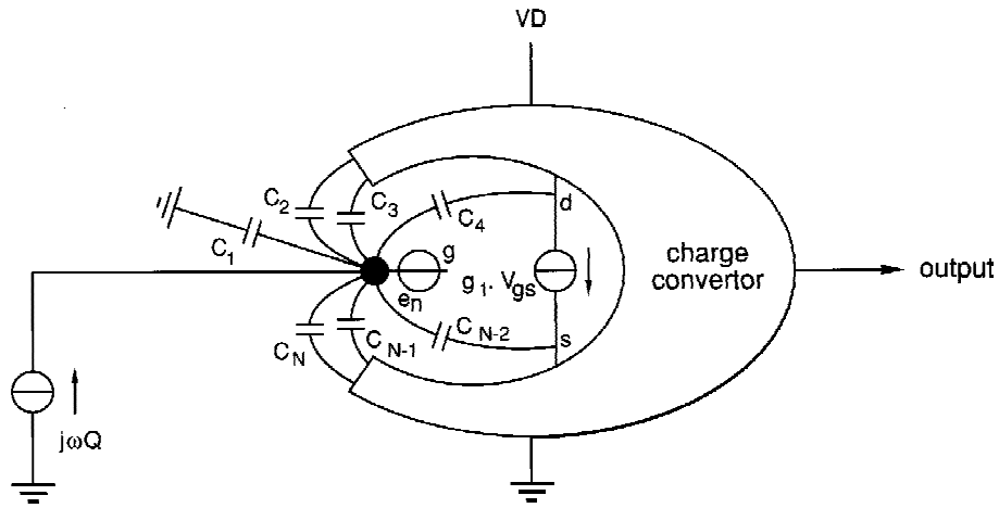
Figure 2.4a: General scheme of a capacitive detection node with a MOS transistor as the first stage of the charge-converter ( M_1 ). The charge dumped on the detection node is represented by a current source j\omega Q .
