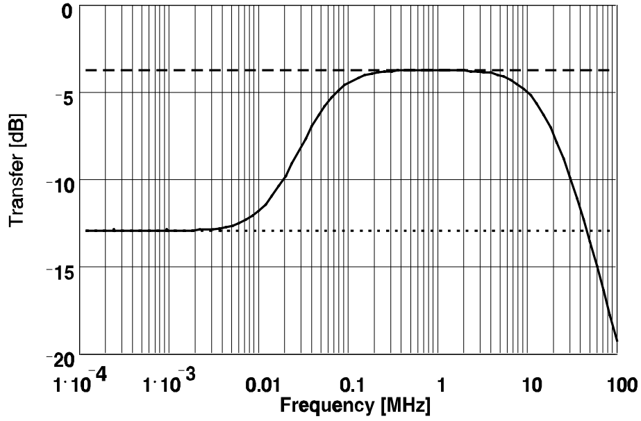
Figure 2.3: The transfer function between the current source gate and the output for a reset FET channel resistance of 300 MΩ. The dotted and the dashed lines are the asymptotic values and their difference is the value of \Theta_n = C_{tol}/C_{det} .
