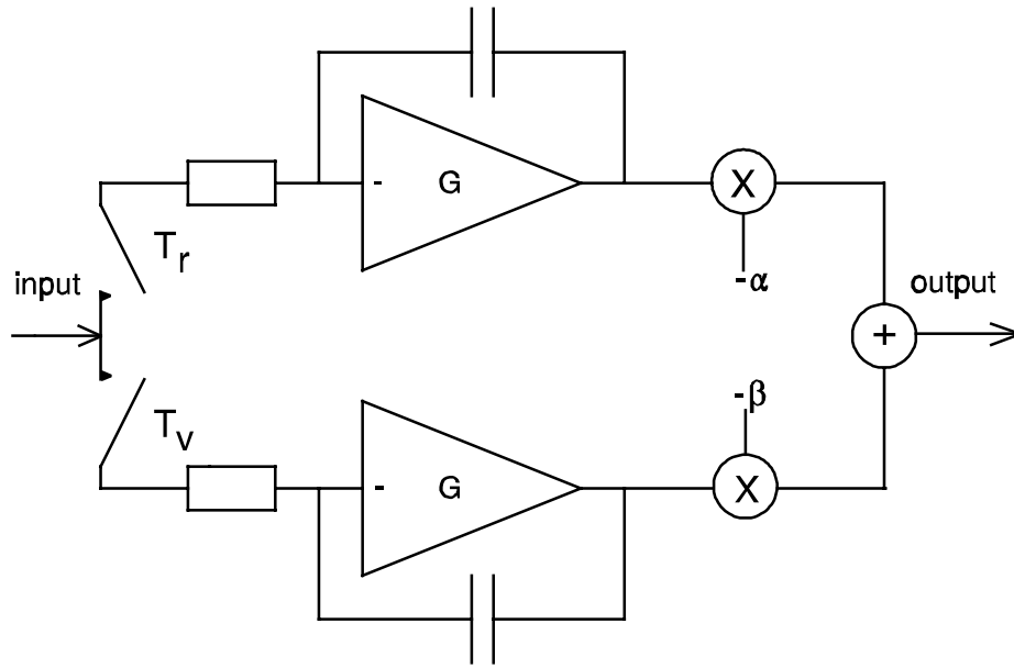
Figure 4.4: The matched filter for the white noise case.
