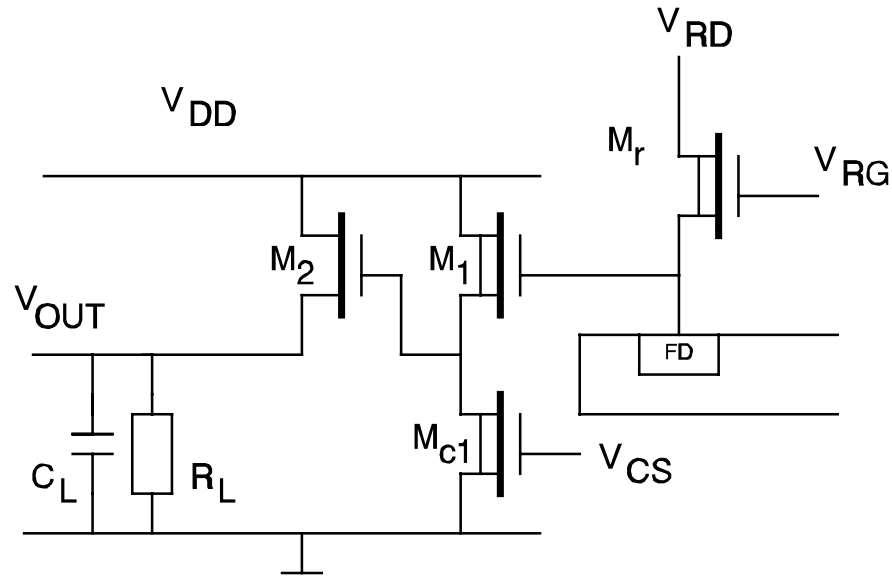
Figure 2.1: A typical on-chip amplifier for CCD imagers, with a floating diffusion detection node.
