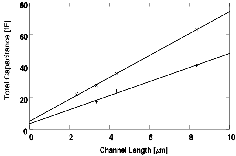
Figure 3.12b: Total capacitance C_{\text{tot}} as a function of the channel length L_1 , for fixed channel width W_1 , for surface channel (x) and buried channel (+) transistors.
