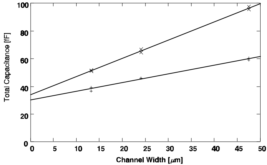
Figure 2.10: The measured total capacitance of the detection node C_{\text{tot}} as a function of channel width W_1 and with the channel length L_1 ((x): 8.7\mu\text{m} and (+): 3.2\mu\text{m} ) as a parameter. The solid lines are least square fits.
