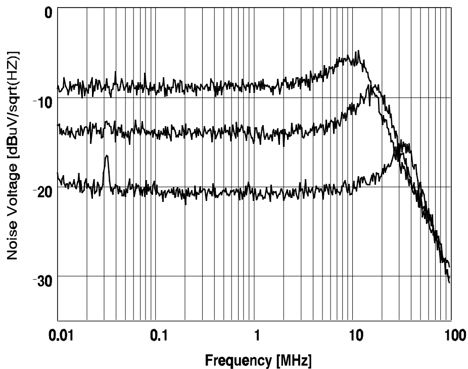
Figure 5.14: The voltage noise spectral density for 3 values of the feedback resistor: upper trace R=34\ \text{M}\Omega , middle trace R=11\ \text{M}\Omega , and lower trace R=2.8\ \text{M}\Omega
