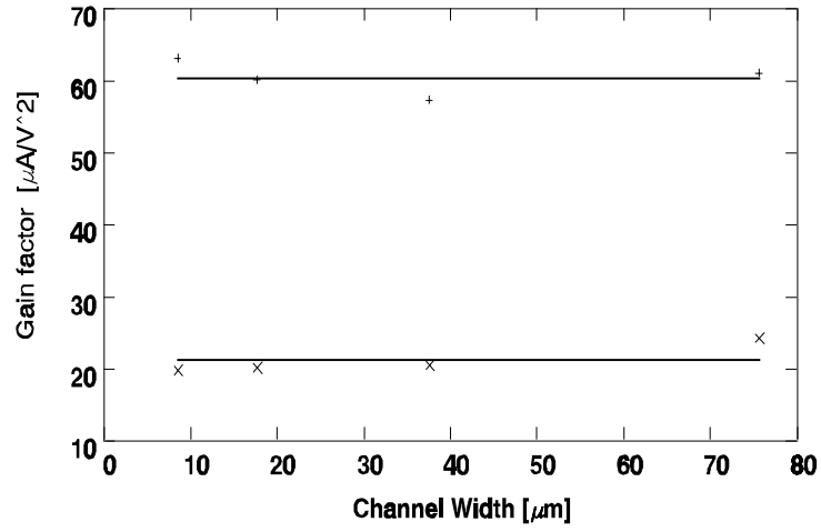
Figure 3.9a: Gain factor \mu_n C_{\square} of a buried channel (x) and surface channel (+) transistor as a function of channel width W_1 . The channel length L_1 and bias current I are fixed.
