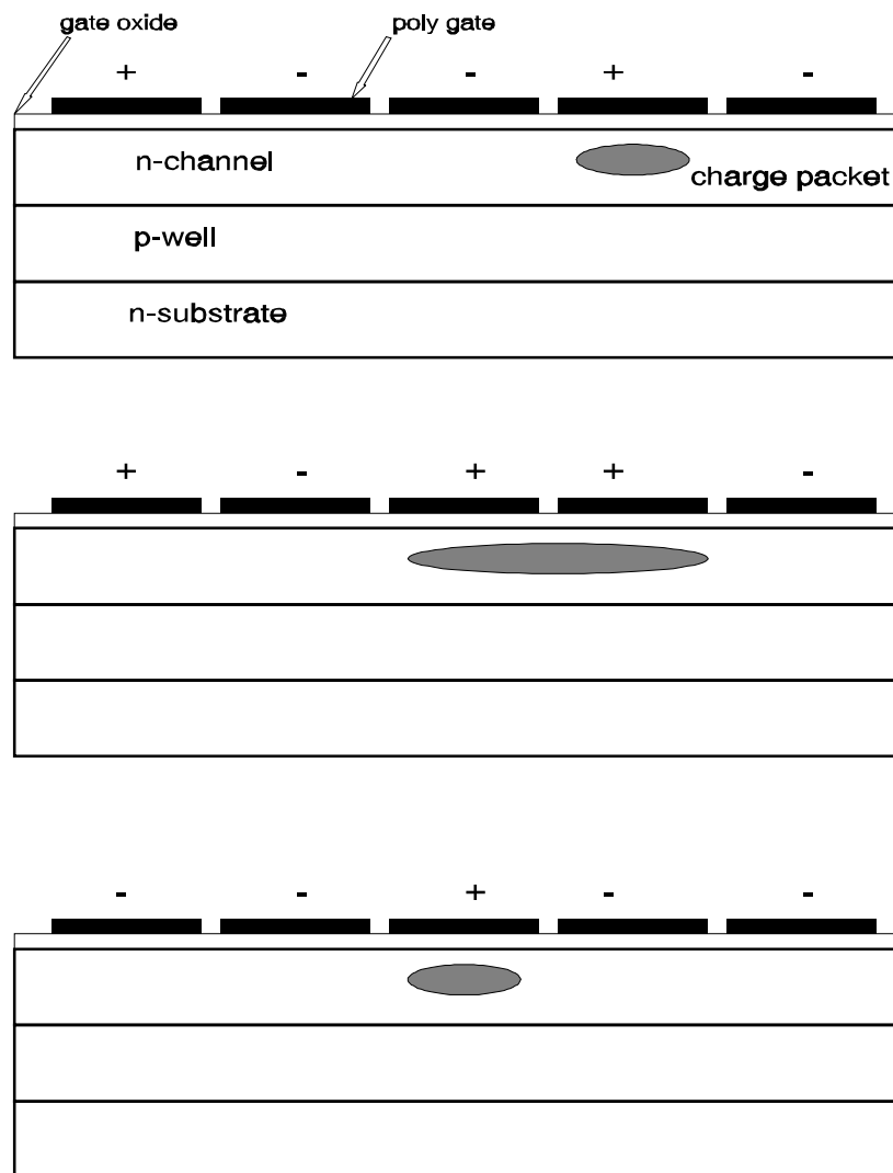
Figure 1.2: Cross section of a CCD, showing the transport of electron charge packets. The charge packet is transported from right to left.
