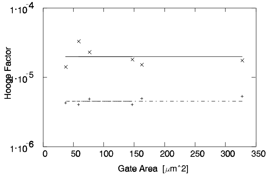
Figure 3.7: Hooge's factor \alpha_H for the 1/f noise generated in buried channel (+) or surface channel (x) detection node transistors.
