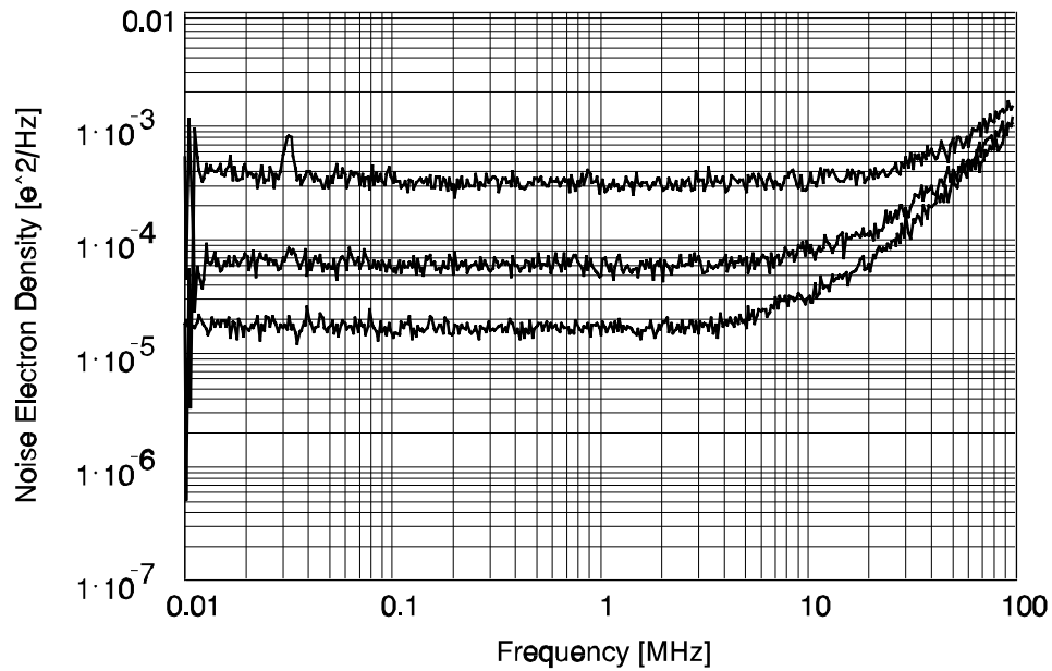
Figure 5.16: The noise spectral density in [ e^2/\text{Hz} ] for R=34\text{ M}\Omega (lower trace), R=11\text{ M}\Omega (middle trace), and R=2.8\text{ M}\Omega (upper trace).
