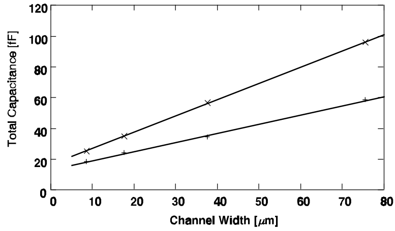
Figure 3.12a: Total capacitance C_{\text{tot}} of the detection node transistor as a function of the channel width W_1 with fixed channel length L_1 , for the surface channel (x) and buried channel (+) cases.
