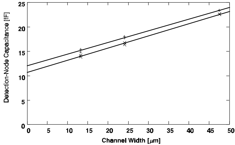
Figure 2.9: The measured detection node capacitance C_{det} as a function of channel width W_1 with the channel length L_1 ( (x) : 8.7\mu\text{m} and (+) : 3.2\mu\text{m} ) as a parameter. The solid lines are least square fits.
