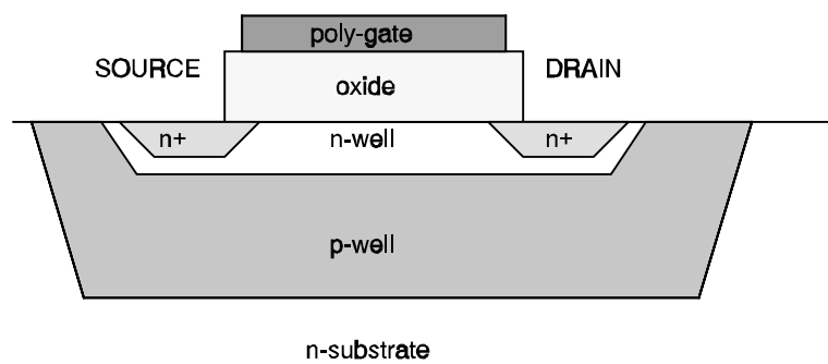
Figure 3.4: Cross sectional view of an n-type buried channel MOS transistor.
