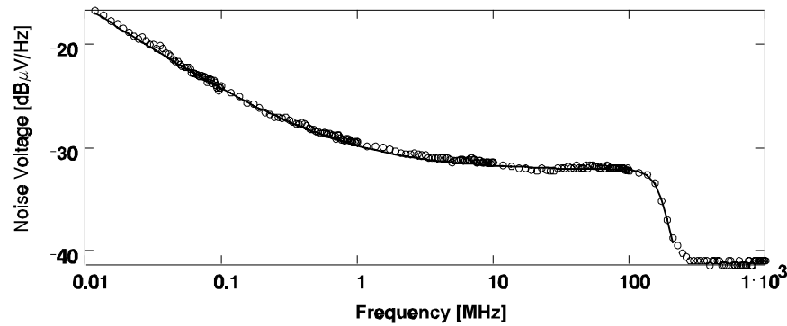
Figure 2.18: Noise spectral density of the FT8-HDTV on-chip amplifier with its low noise and high bandwidth. Dots are measurements and the solid line is a least square fit.
