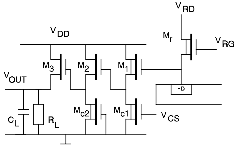
Figure 2.17: Shown is a schematic view of the on-chip amplifier of the FT8 HDTV imager.
