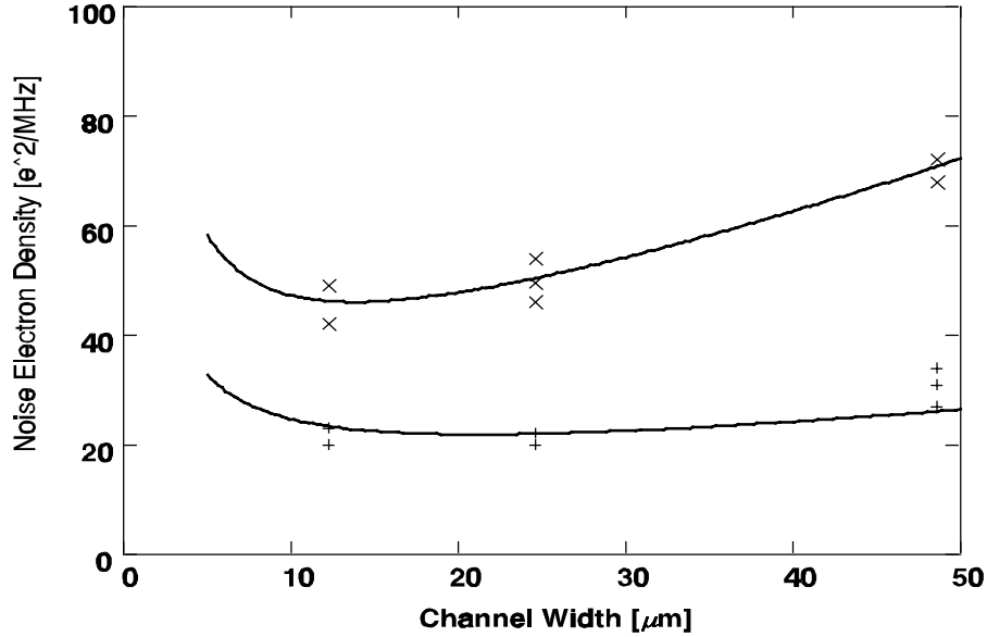
Figure 2.13: The Noise Electron Density of the thermal noise as a function of the channel width W_1 with the channel length L_1 as a parameter ( (x) : 8.7\text{ }\mu\text{m} and (+) : 3.2\text{ }\mu\text{m} ). The bias current is 100\text{ }\mu\text{A} . The solid lines are calculated results according to equation (2.38).
