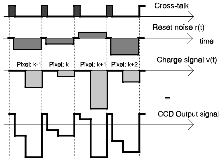
Figure 4.1: The CCD output signal decomposed into three sources.
